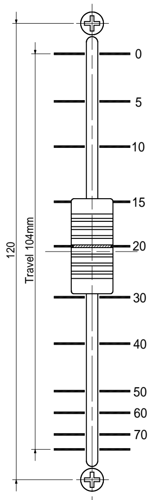
104mm Audio taper
