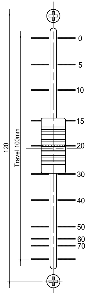
100mm Audio-PG(AP) taper
