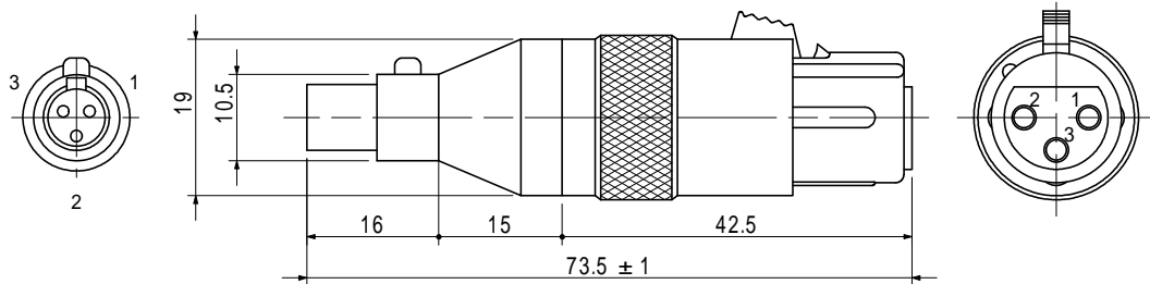
MiXL3-22XLR
